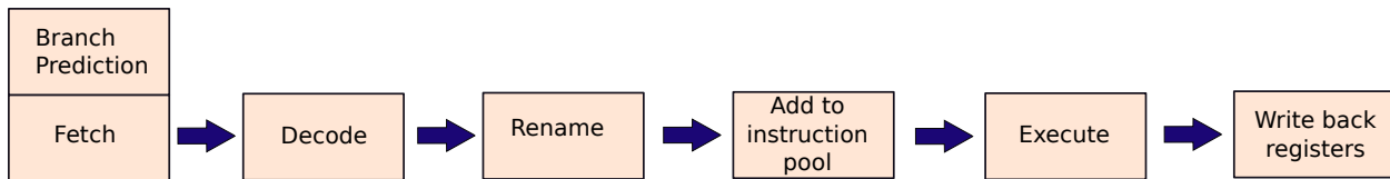
Figure 2.23: The OOO pipeline (as explained till now)
