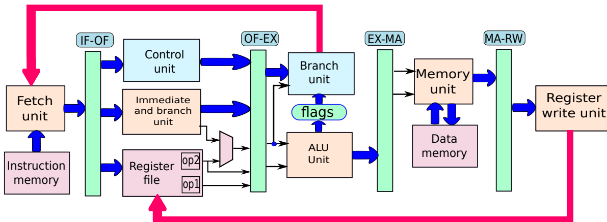
Figure 2.6: 5-stage pipeline with latches between stages
