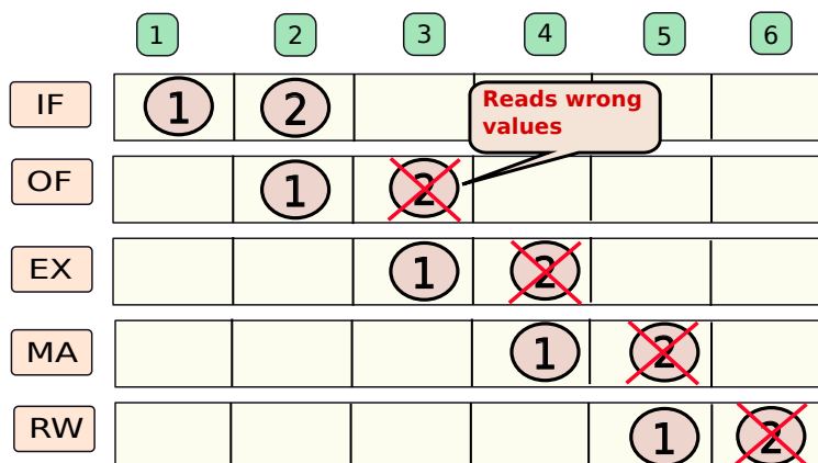
Figure 2.7: Graphical view of a data hazard
