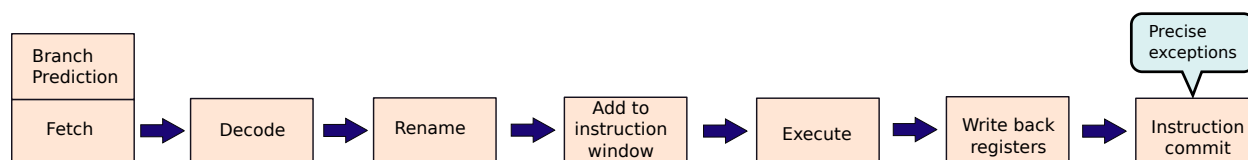
Figure 2.24: The OOO pipeline
