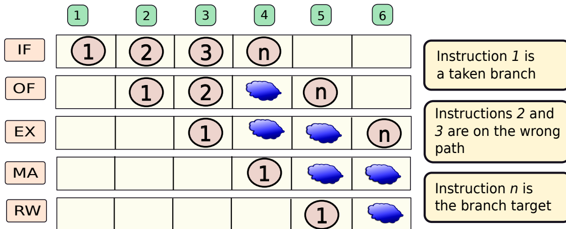
Figure 2.10: Nullifying two instructions on the wrong path
