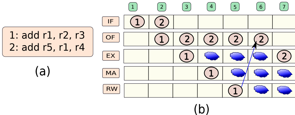
Figure 2.11: Example of a stall
