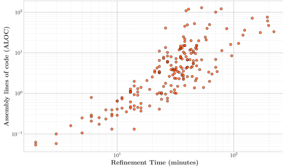
Figure 6.6: Scatter plot of refinement time (in minutes) vs assembly lines of code (ALOC). Both axes are logarithmically scaled.
