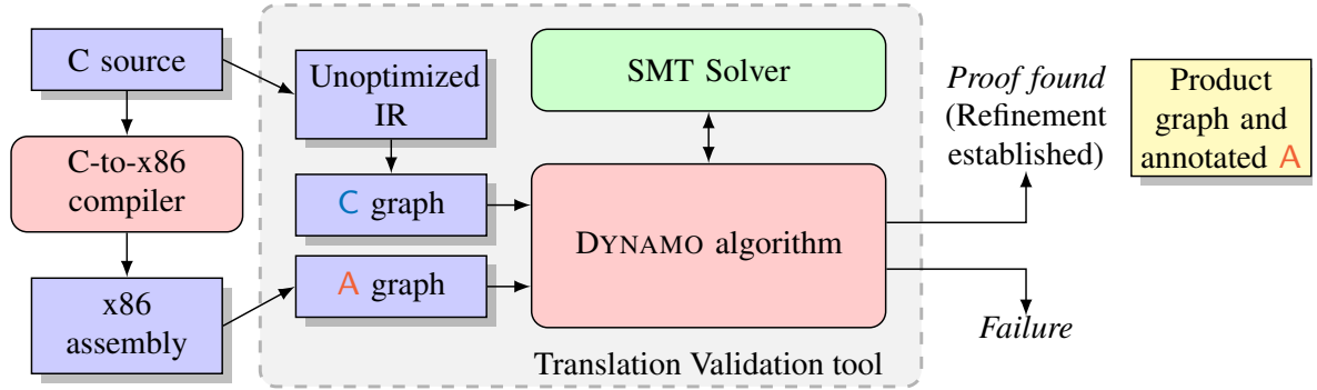
Figure 1.5: High-level components and flow of our translation validation approach.
