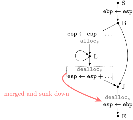
(b) Abbreviated CFG of GCC compiled assembly
