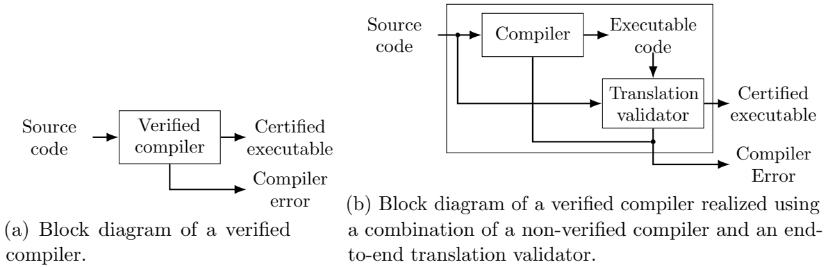
Figure 1.1: Two ways of obtaining a certified executable from an input source code. The certified executable is guaranteed to have identical semantics as the input source code.
