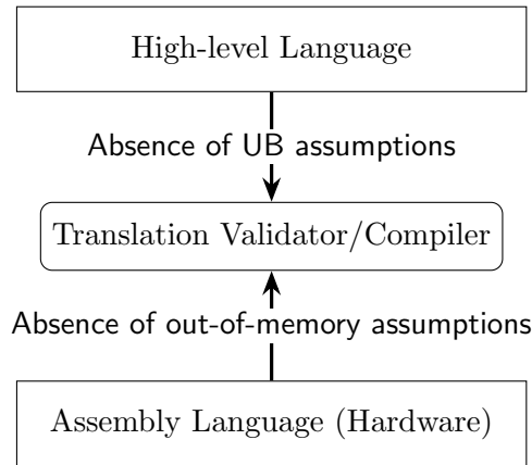
Figure 1.4: Conceptual representation of the flow of information from high-level source program and the low-level assembly program to the compiler/translation validator.
