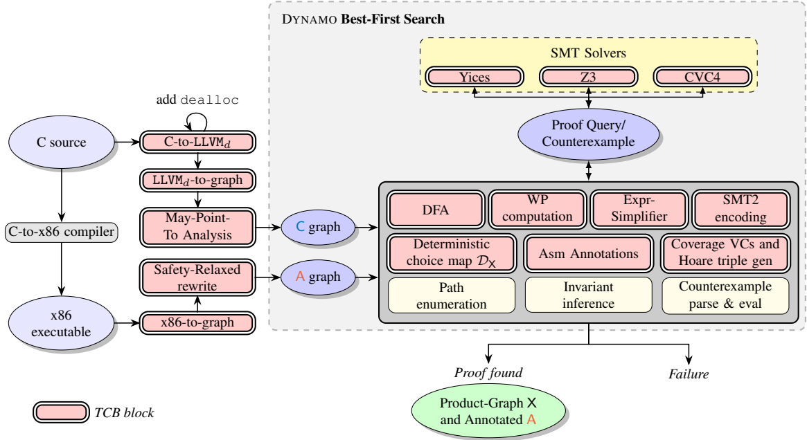
Figure 6.1: High-level components of DYNAMO implementation. Trusted Code Base (TCB) blocks have double border and a red background.
