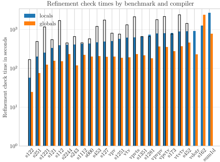
Figure 6.5: Comparison of running times of TSVC benchmarks with exactly same code modulo allocation strategy. Y-axis is logarithmically scaled.
