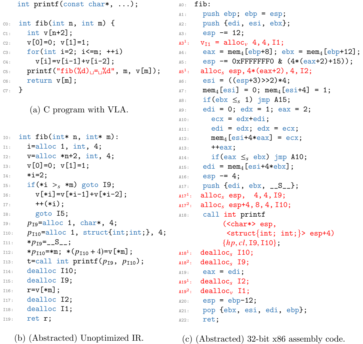
Figure 4.4: Reproduced C program and its unoptimized IR and assembly from fig. 2.1.
