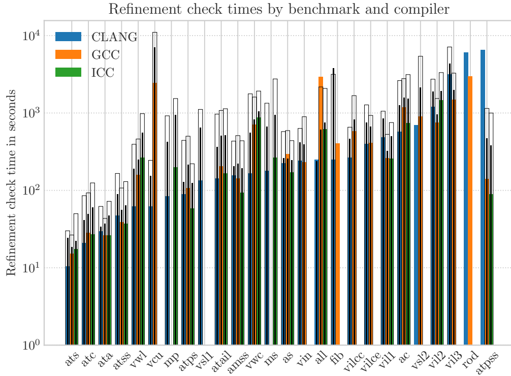
Figure 6.2: Comparison of running times of procedures in table 6.1 with full-interval (filled bars), partial-interval (thick black lines), and full-array (empty bars) encoding. Y-axis is logarithmically scaled.
