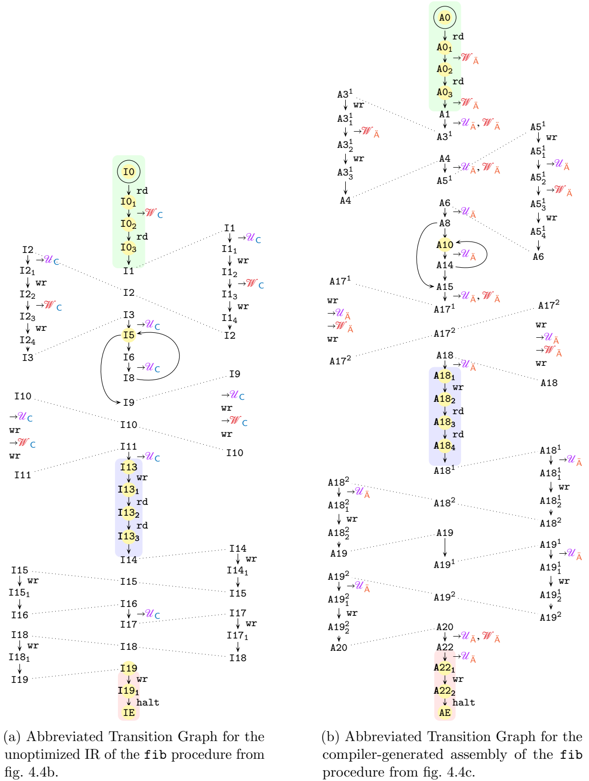
Figure 4.5: Abbreviated Transition Graphs for the unoptimized IR and assembly of the fib procedure from fig. 4.4.
