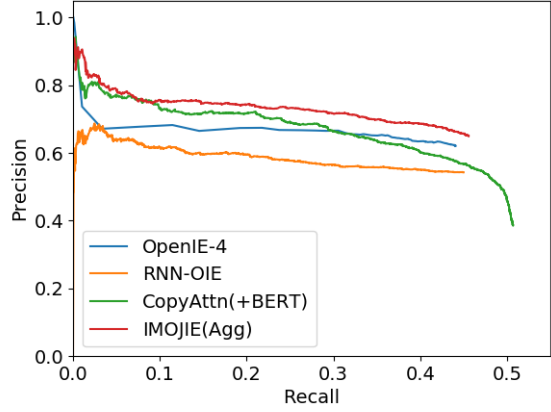
Figure 3: Precision-Recall curve of OpenIE Systems.
