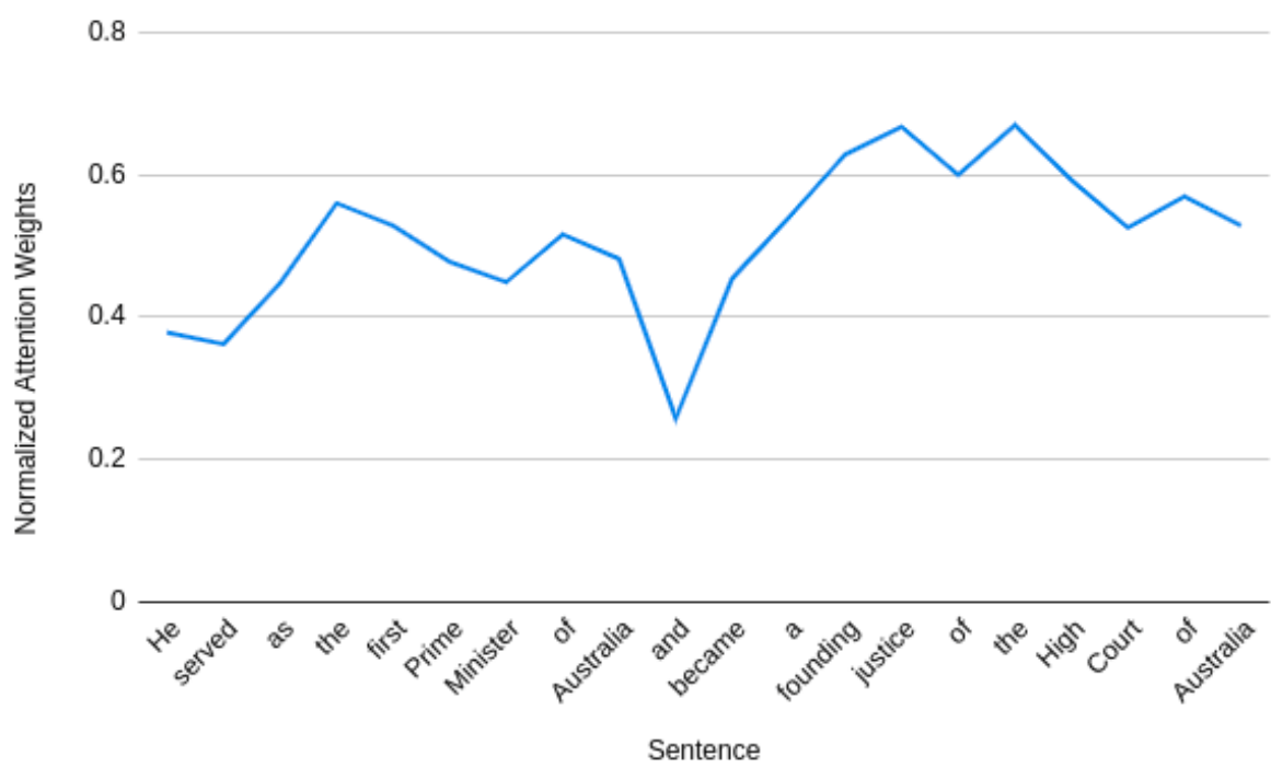
Figure 10: Attention weights for the decoder
