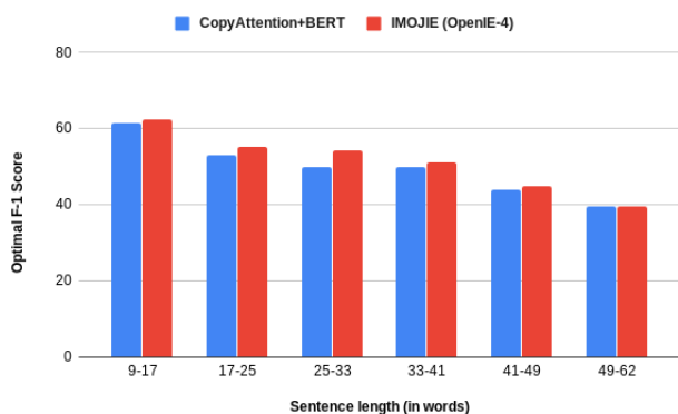
Figure 4: Measuring performance with varying input sentence lengths
