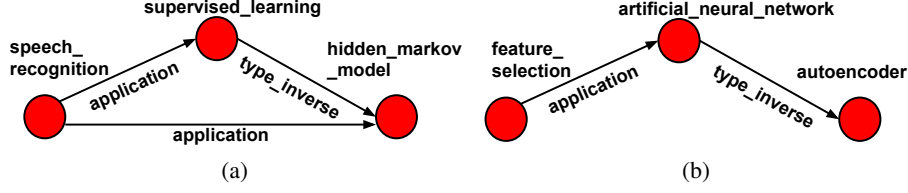
Fig. 1: Examples of meta-paths for application relation. (a) The meta-path \langle \text{application}, \text{type\_inverse} \rangle exists between speech_recognition and hidden\_markov\_model . (b) feature\_selection and autoencoder are not related by application relation but still it can be inferred because of the existence of the same meta-path \langle \text{application}, \text{type\_inverse} \rangle between them.
