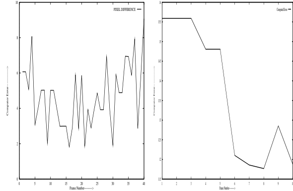
Figure 3: Graph showing error for (a)Football sequence (b)cricket sequence
