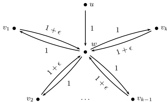
Figure 1: Tightness. Let the graph be G . All other edges in this graph have 0 weight. The weight of the maximum weight branching in G is k + 1 while the maximum weight branching in G_k is k + \epsilon . As \epsilon \rightarrow 0 we get a \frac{k}{k+1} factor.
