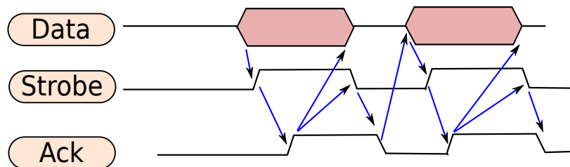
Figure 12.20: Timing diagram of a strobe based asynchronous communication system with handshaking
