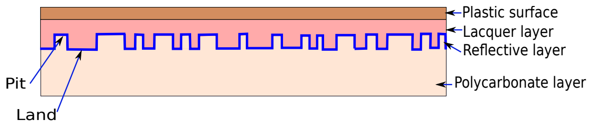
Figure 12.39: Optical disk layers
