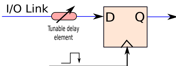
Figure 12.14: The receiver of a mesochronous bus
